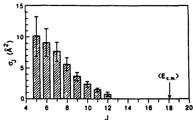
Fig. 11. Absolute integral cross sections (in \text{\AA}^2 ) for scattering of thermal HCl into a final J level
